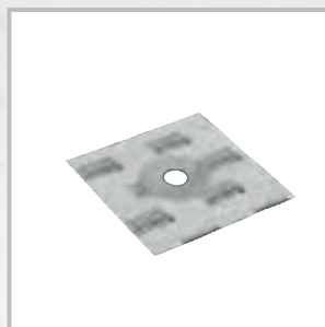
■ LUX ELEMENTS®-DRY-DBDZM – Expansion zone sleeve On PU basis. Two different sizes having a central expansion zone to enable pipes of different external diameters to be sealed. Installation in combination with DRY-ASK.
