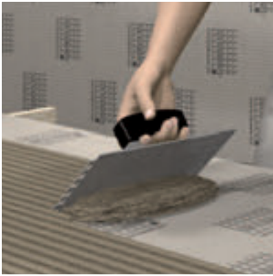
Full-surface application of fixing adhesive COL-AK with the notched trowel for wall and floor applications.
