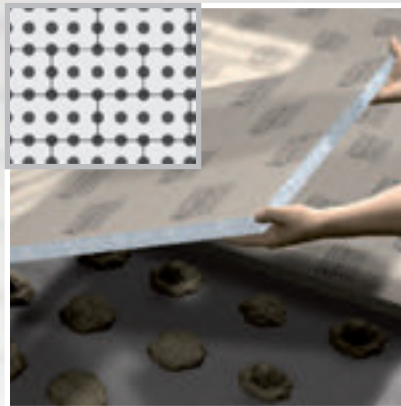
Floor application from ELEMENT-EL 30: dot spacing COL-AK (25 – 36 dots per m 2 ) approx. 20 cm. Place panels in bond onto the adhesive and press on (cross joints not allowed!).
