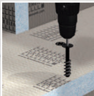
Plastic screw plugs FIX-SD enable the connection of hard foam support elements to one another.
