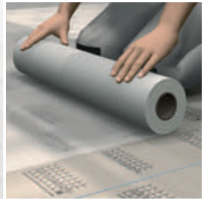
A particularly broad reinforcement fabric ARM-600, that is embedded on the surface and then levelled out with fixing adhesive COL-AK is suitable for use on floors and larger surfaces.
