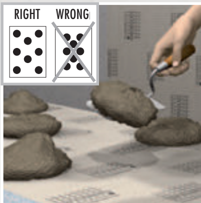
Wall application from ELEMENT-EL 6: For height compensation in case of uneven substrates, apply the fixing adhesive COL-AK pointwise using dots of adhesive (8–10 dots per m 2 ) auftragen.
